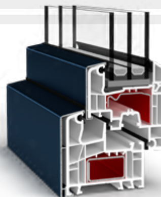
ALUMINIUM COVER
