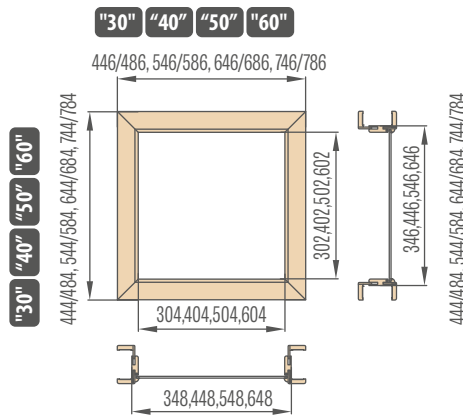
Top sidelights for adjustable door frame of double-leaf rebated doors, architrave 6 cm / architrave 8 cm
