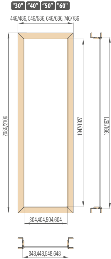
Sidelights for doors for adjustable rebated door frame, architrave 6 cm / architrave 8 cm
