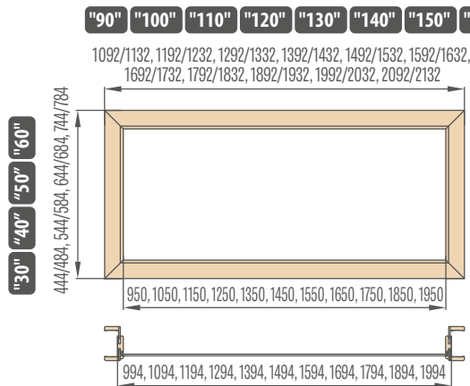
Top sidelights for adjustable door frame of double-leaf rebated doors, architrave 6 cm / architrave 8 cm
