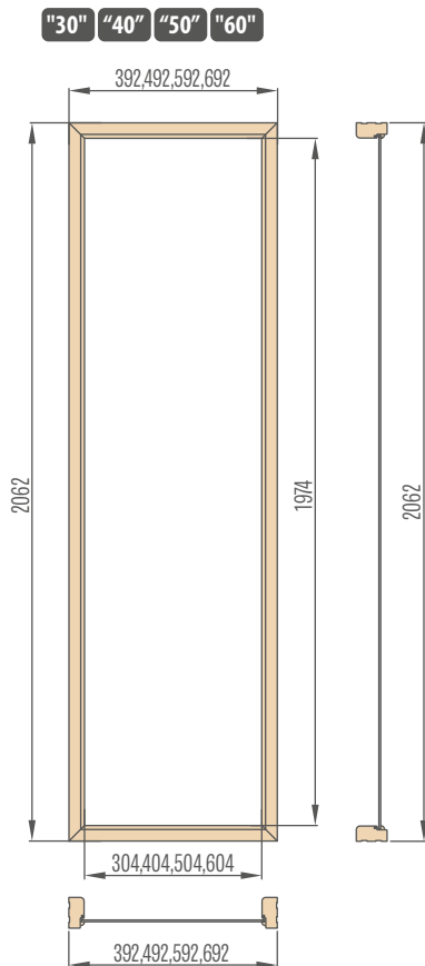
Side sidelights for fixed frame
