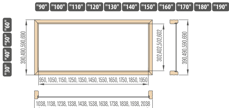
Top sidelights for fixed frame of double-leaf doors
