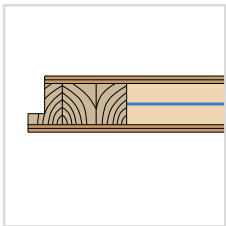
46 mm door leaf reinforced with steel sheet
