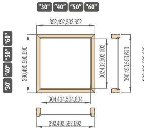
Corner sidelights for fixed frame
