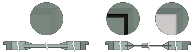
WERBENA 1, 2, 3 beveled strip at 16 mm panel
