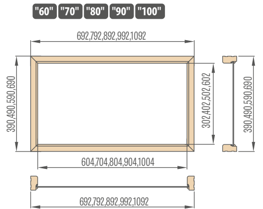
Top sidelights for fixed frame of single-leaf doors
