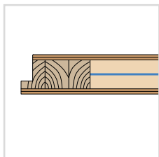
DOOR LEAF 46 mm Steel sheet reinforced
