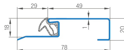
STAINLESS STEEL SHEET THRESHOLD
