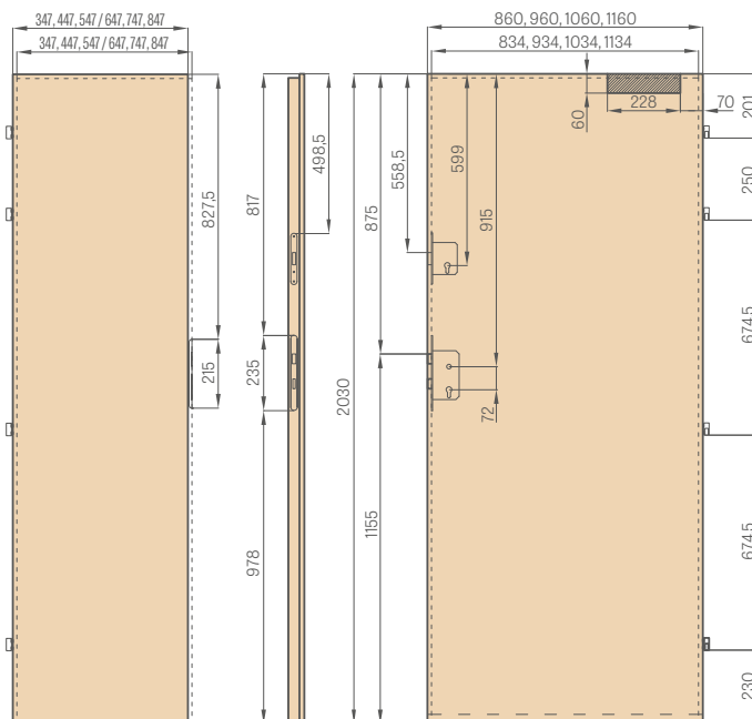
Side panel / inactive door leaf
